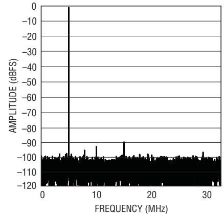
LTC2172-12: 8k Point FFT, f_{IN} = 5\text{MHz} -1dBFS, 65Msps
