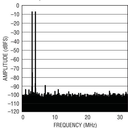
LTC2172-12: 8k Point 2-Tone FFT, f_{IN} = 68\text{MHz}, 69\text{MHz} , -1dBFS, 65Msps
