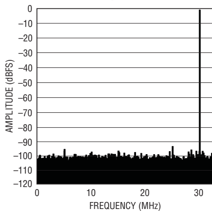
LTC2172-12: 8k Point FFT, f_{IN} = 30\text{MHz} -1dBFS, 65Msps
