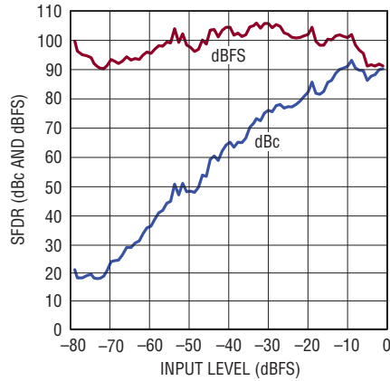
LTC2172-12: SFDR vs Input Level, f_{IN} = 70\text{MHz} , 2V Range, 65Mps
