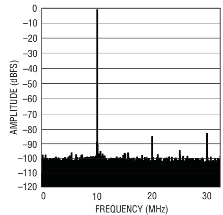
LTC2172-12: 8k Point FFT, f_{IN} = 140\text{MHz} -1dBFS, 65Msps
