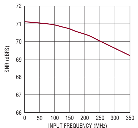
LTC2172-12: SNR vs Input Frequency, -1dBFS, 2V Range, 65Msps
