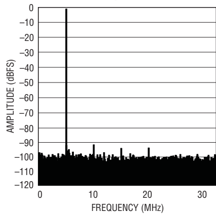
LTC2172-12: 8k Point FFT, f_{IN} = 70\text{MHz} -1dBFS, 65Msps
