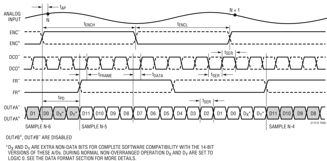
1-Lane Output Mode, 14-Bit Serialization
