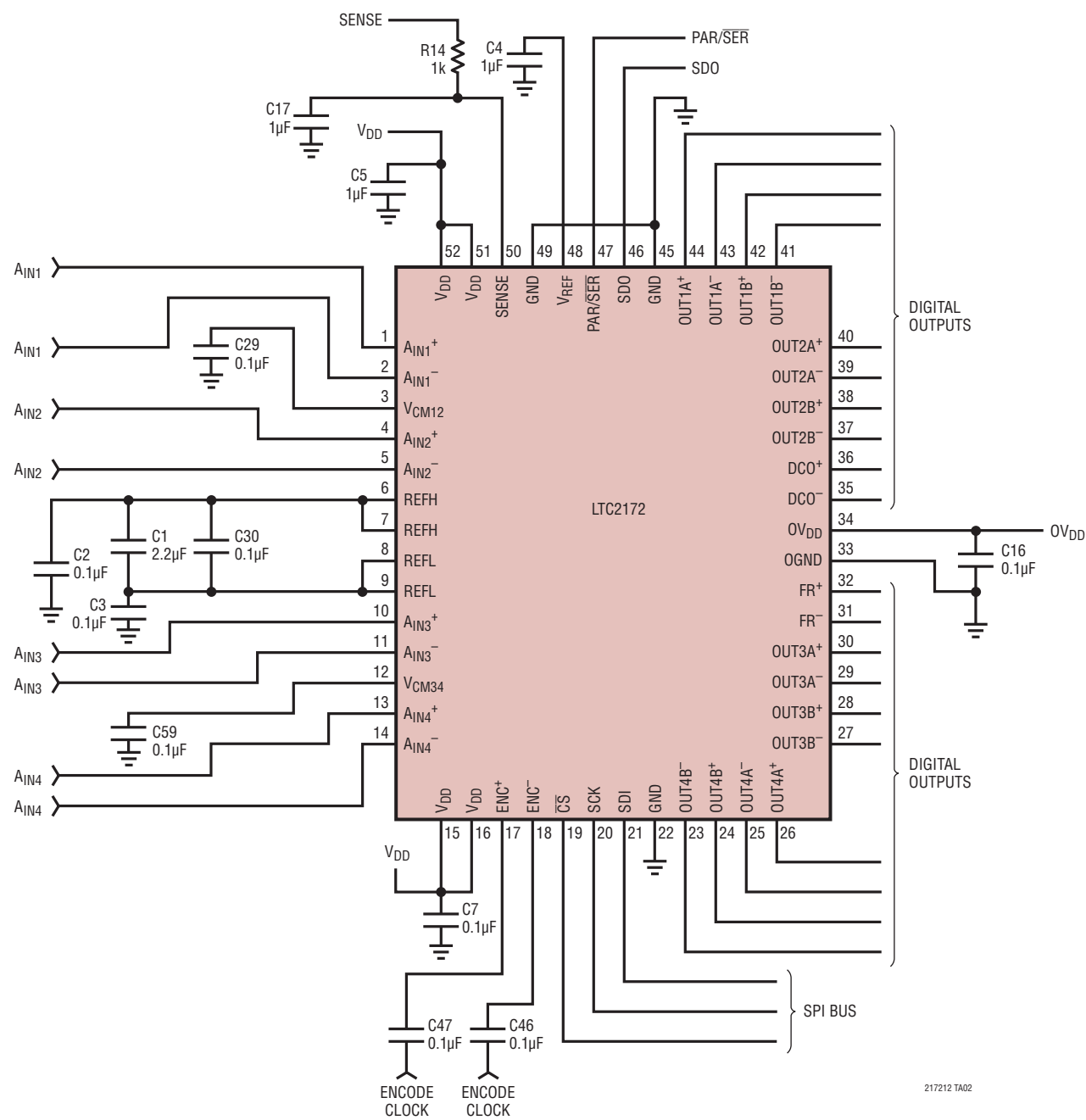
LTC2172 Schematic
