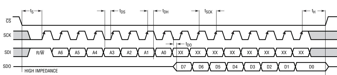
SPI Port Timing (Readback Mode)
